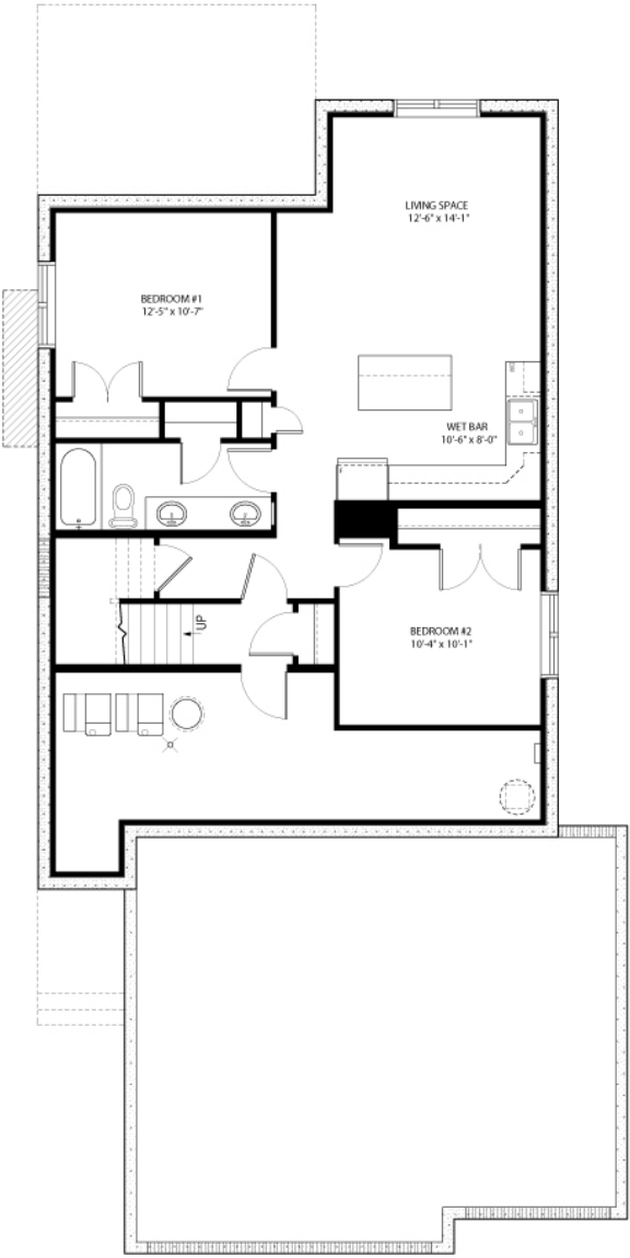
OPTIONAL BASEMENT SUITE PLAN-880sq.ft.
