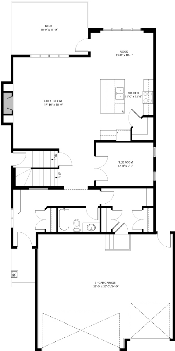
MAIN FLOOR PLAN - 1204 sq.ft.
