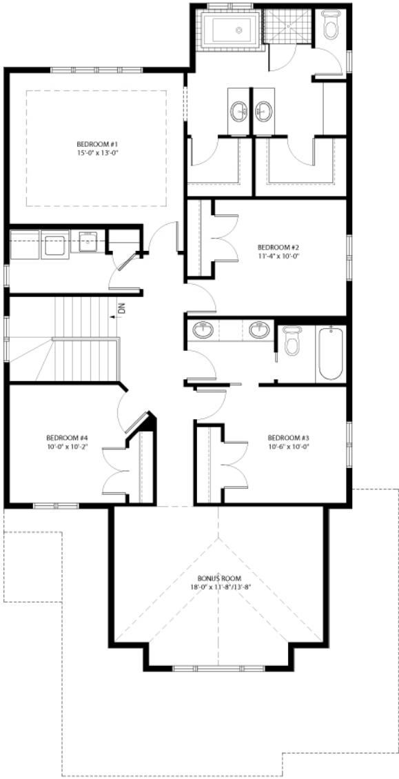
SECOND FLOOR PLAN-1404sq.ft.
