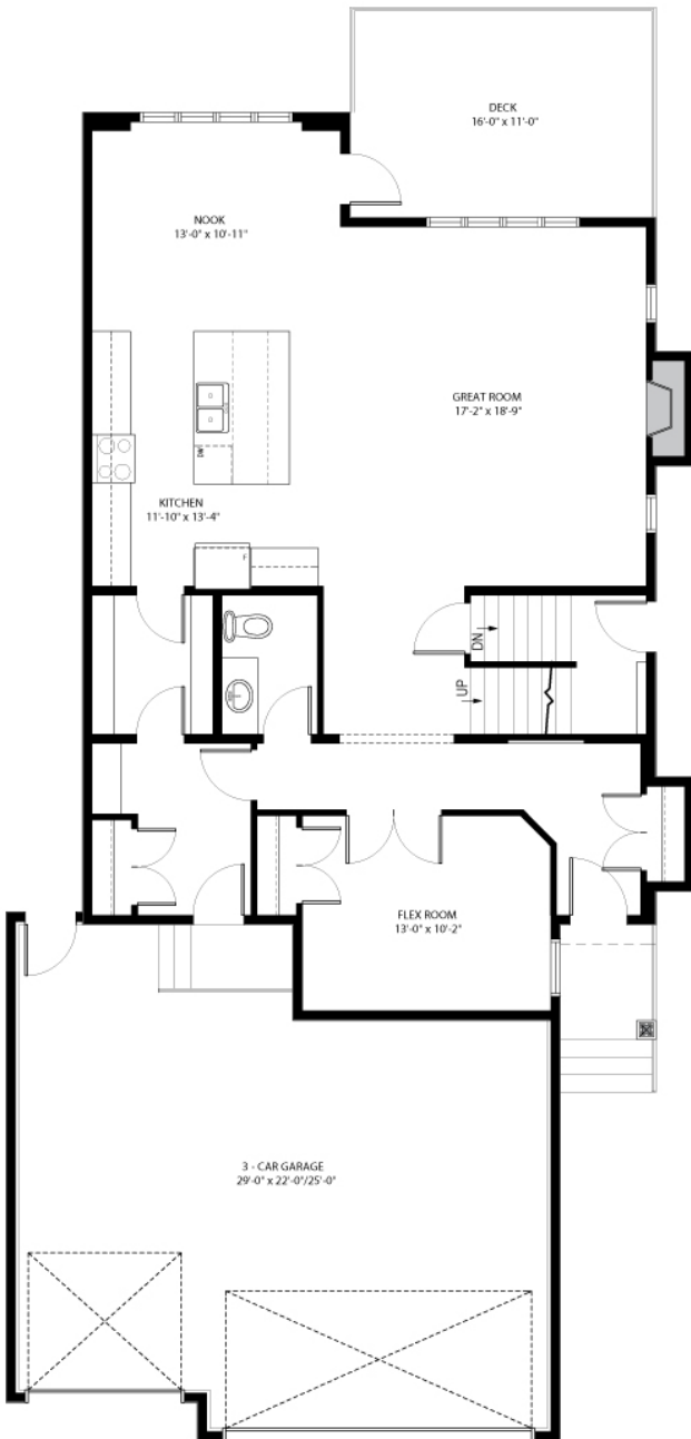
MAIN FLOOR PLAN-1257sq.ft.
